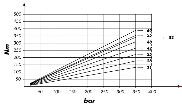
DRIVE TORQUE
