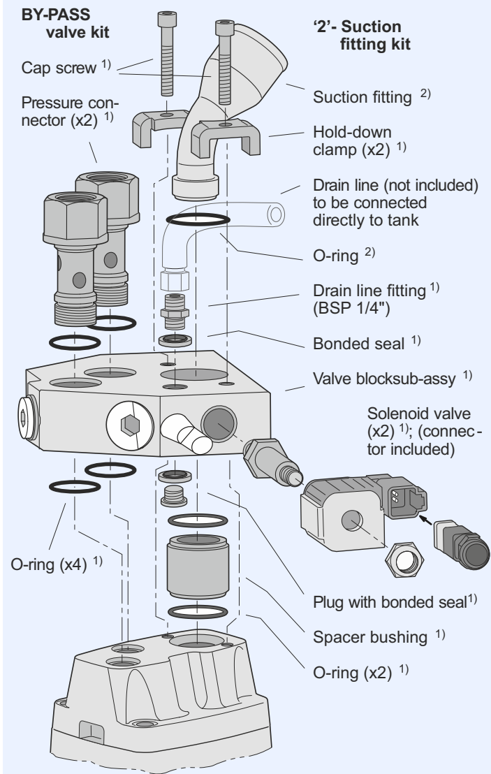
Bypass valve split view with manual override (with pump end cap).
